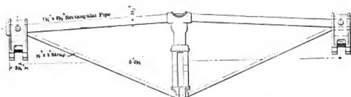
Fig. 4441. Kewaunee Tender Brake Beam with Reversible Struts. Chicago Railway Equipment Co.
